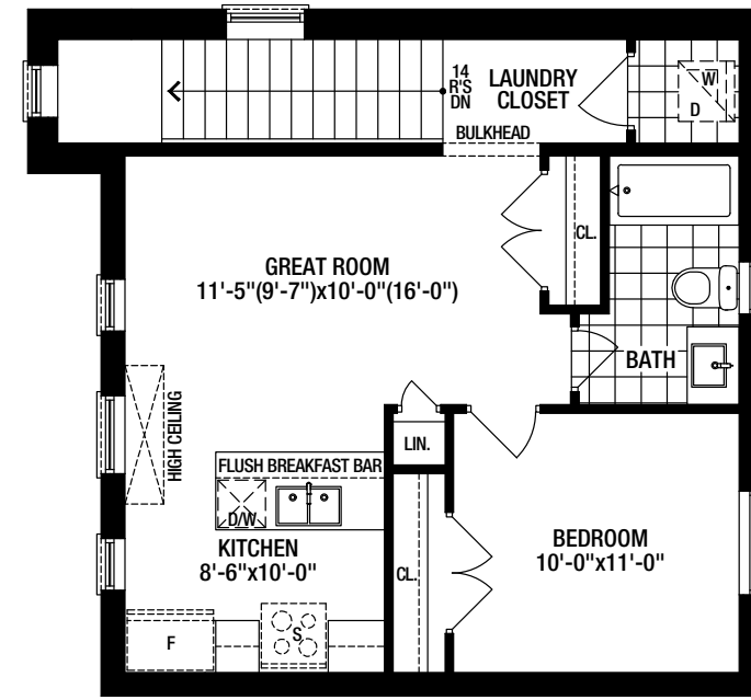
SECOND FLOOR A COACH HOUSE
