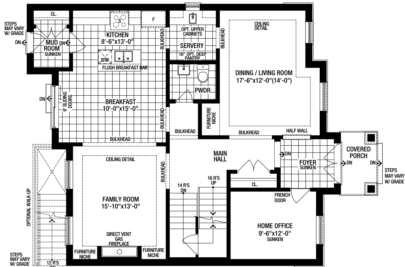
GROUND FLOOR MAIN HOUSE A
