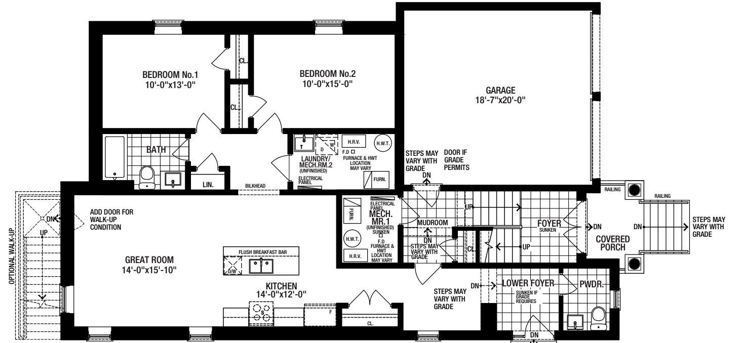
OPTIONAL ACCESSORY BASEMENT FLOOR A
