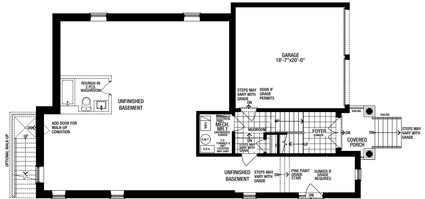
STANDARD BASEMENT FLOOR A
