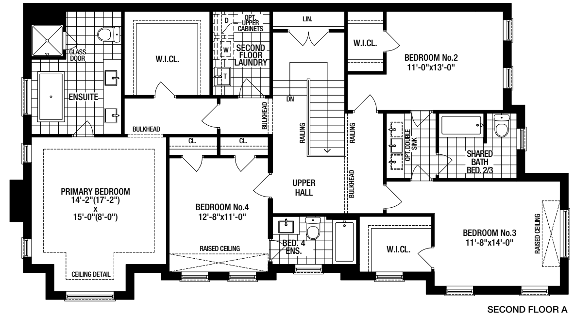
SECOND FLOOR A
