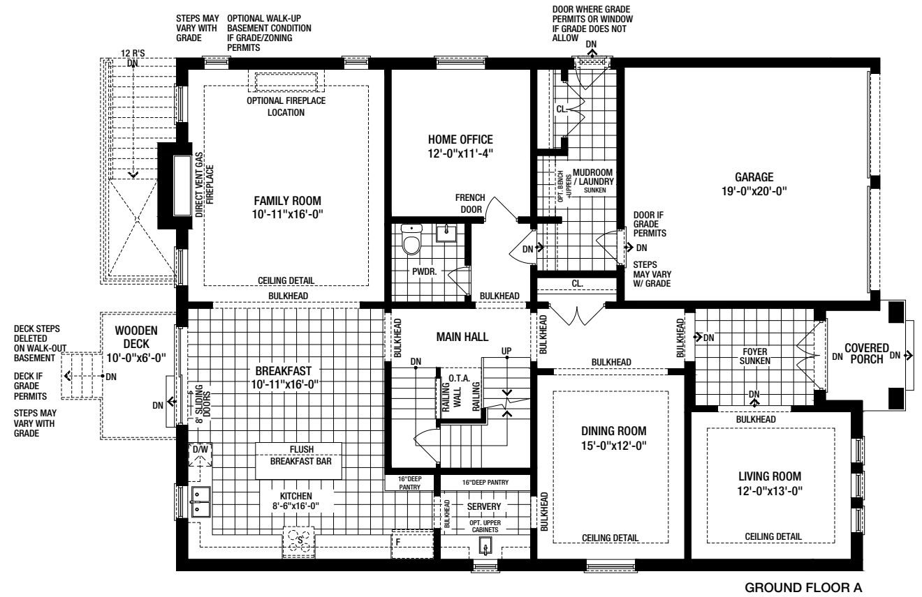
GROUND FLOOR A
