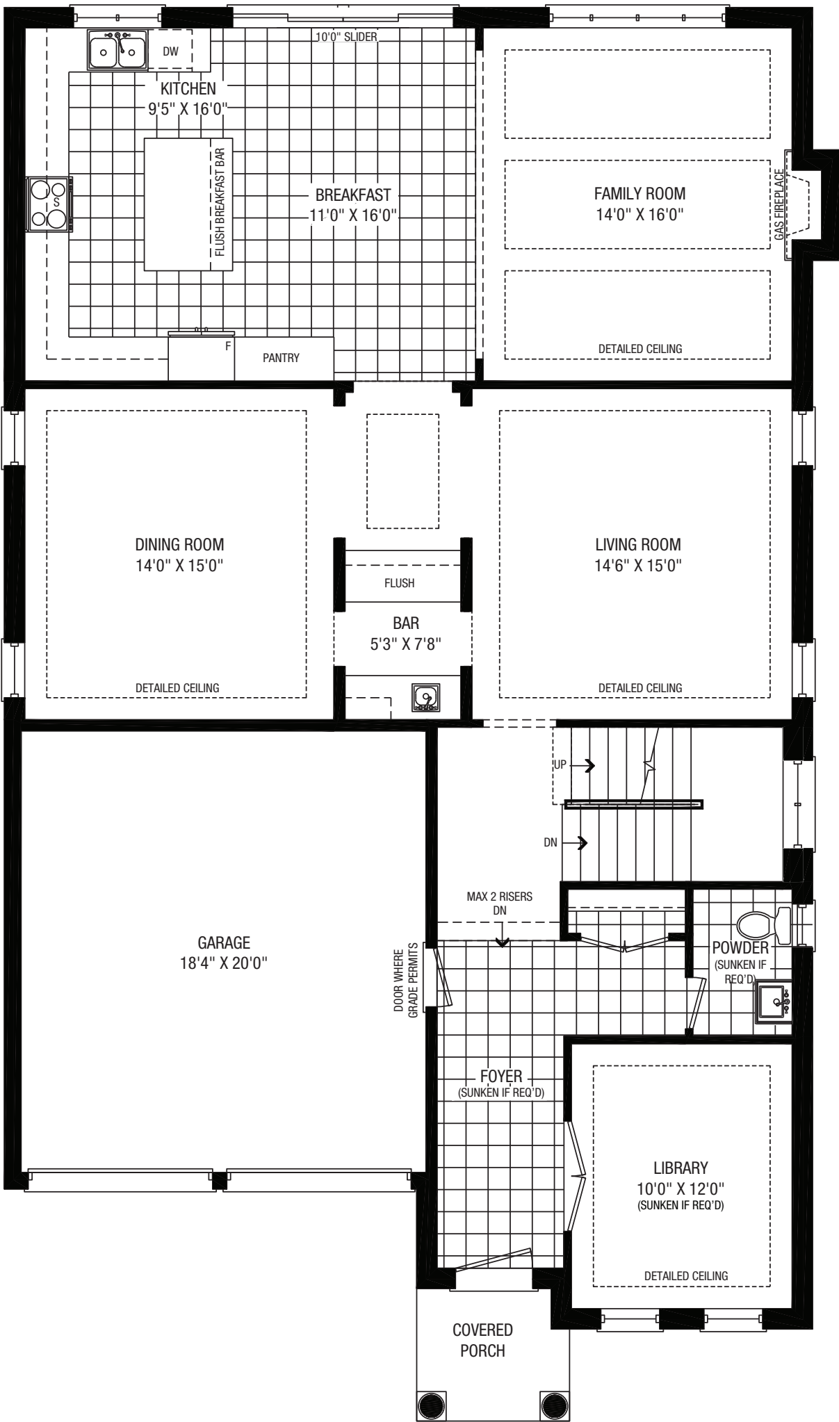
GROUND FLOOR 'A'
