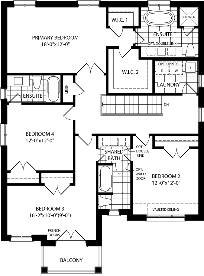
SECOND FLOOR A
