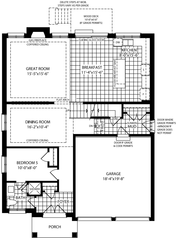
OPTIONAL GROUND FLOOR A 5 BEDROOM
