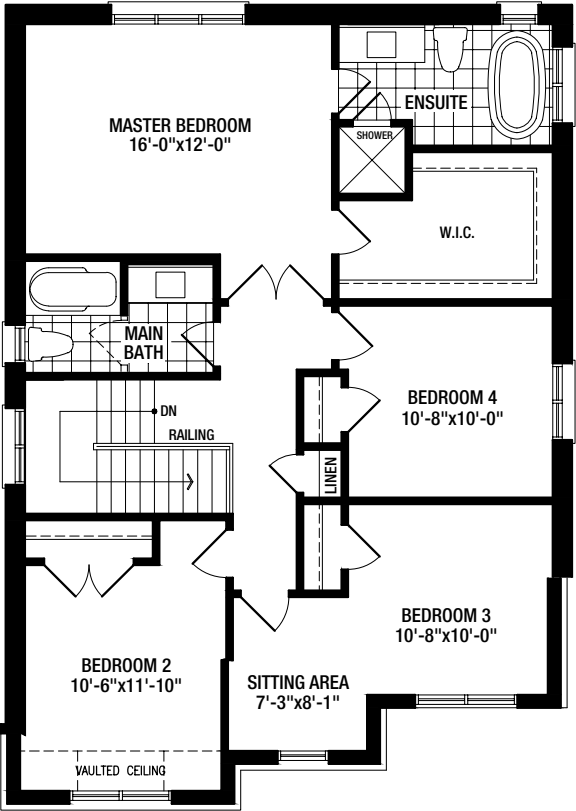
OPTIONAL SECOND FLOOR B 4 BEDROOM
