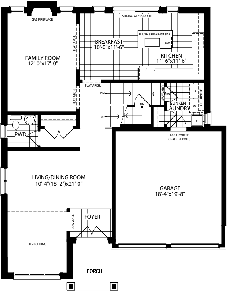
MAIN FLOOR C
