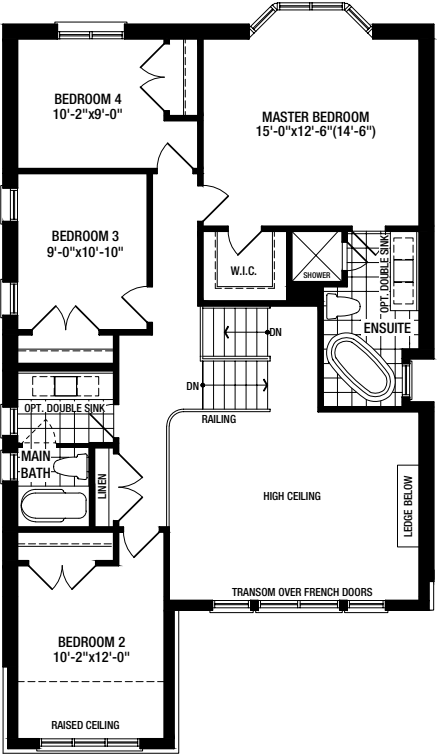
OPTIONAL SECOND FLOOR C 4 BEDROOM
