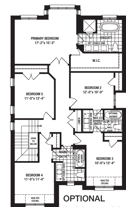
SECOND FLOOR A
