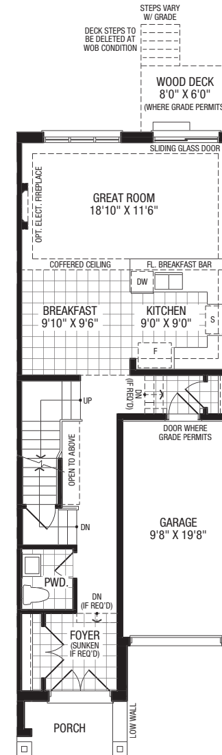
Ground Floor
