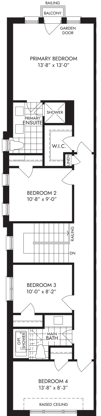
UPPER FLOOR ELEV. C
