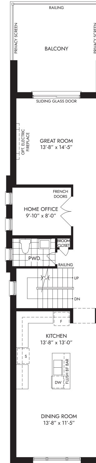
MAIN FLOOR ELEV. C
