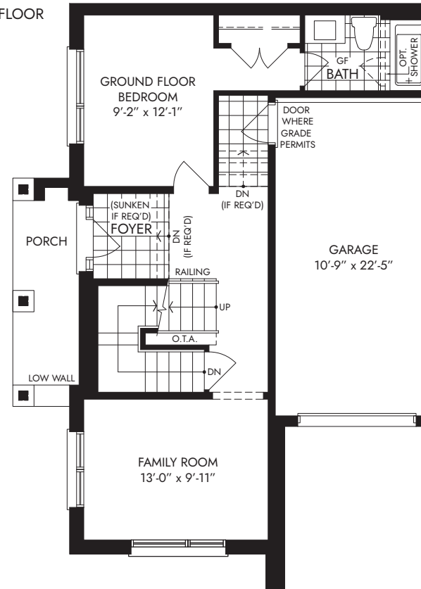
MAIN FLOOR ELEV. C
