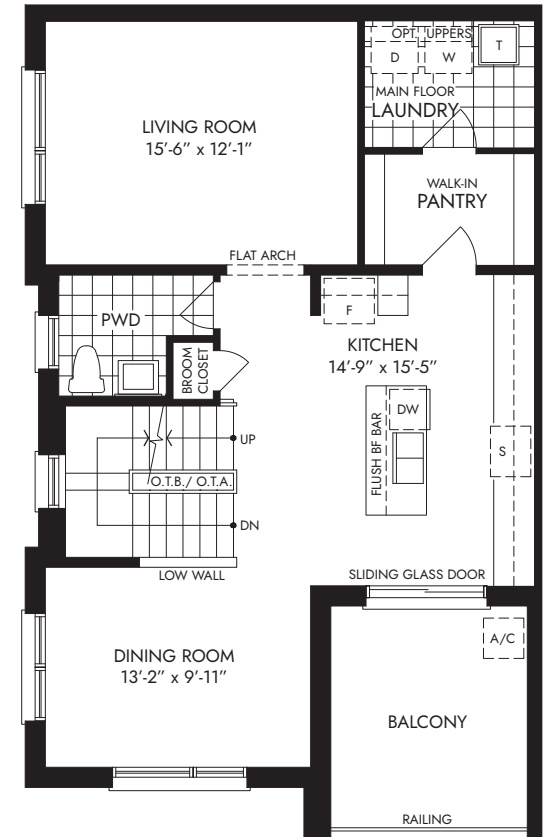
MAIN FLOOR ELEV. C
